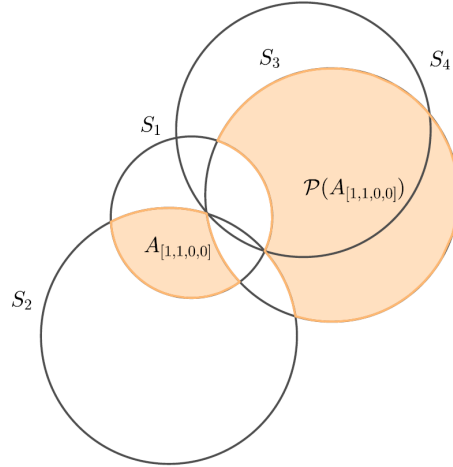
Figure 5: Illustrating Example 6.12 when A_{[0,0,1,1]} \subsetneq \mathcal{P}(A_{[1,1,0,0]}) .
